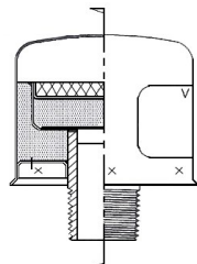
Type DB External Pipe Thread
